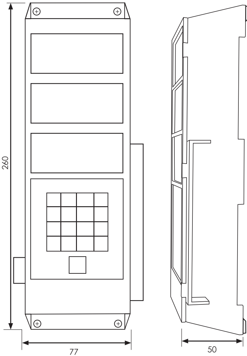
Size of 204EU in mm
