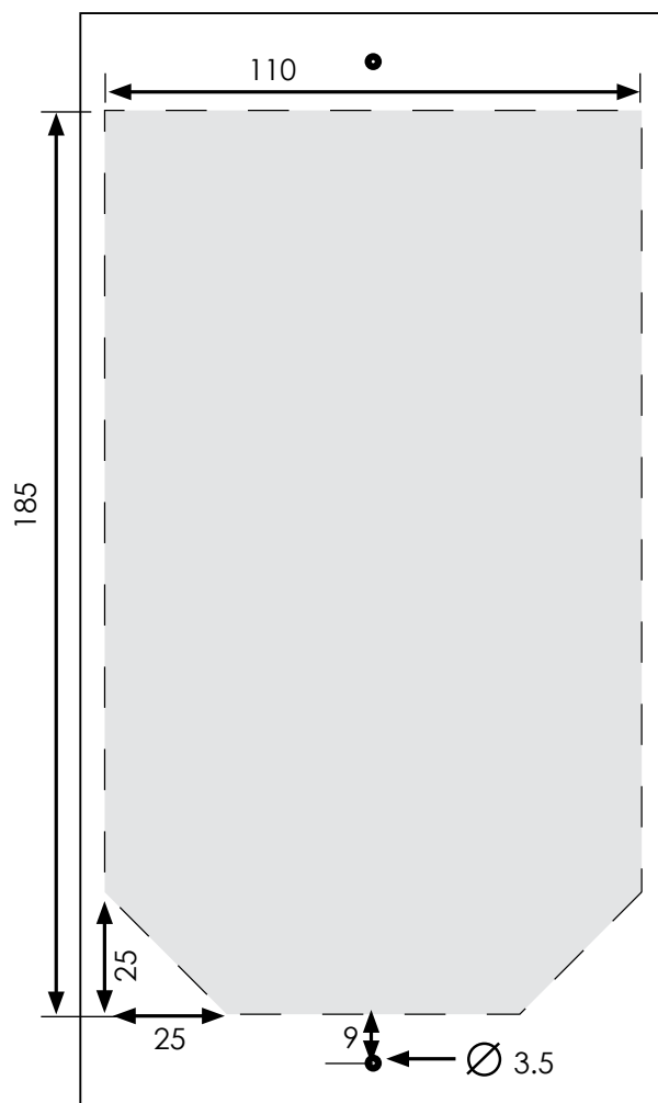
Schema for installation
