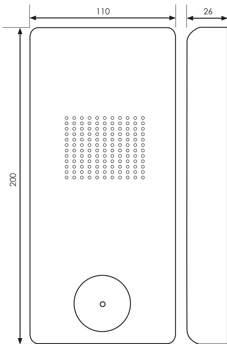
Size of 232EU in mm
